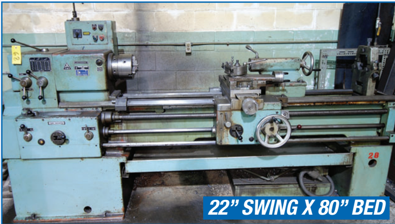
TOS SN50B ENGINE LATHE
